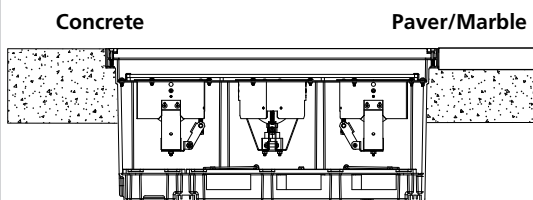
SL-29 In Concrete With Trim Ring
