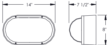
BL-44 THRU 49 TYPICAL FIXTURE DIMENSIONS
