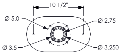
BL-44 THRU 49 MOUNTING DETAIL
