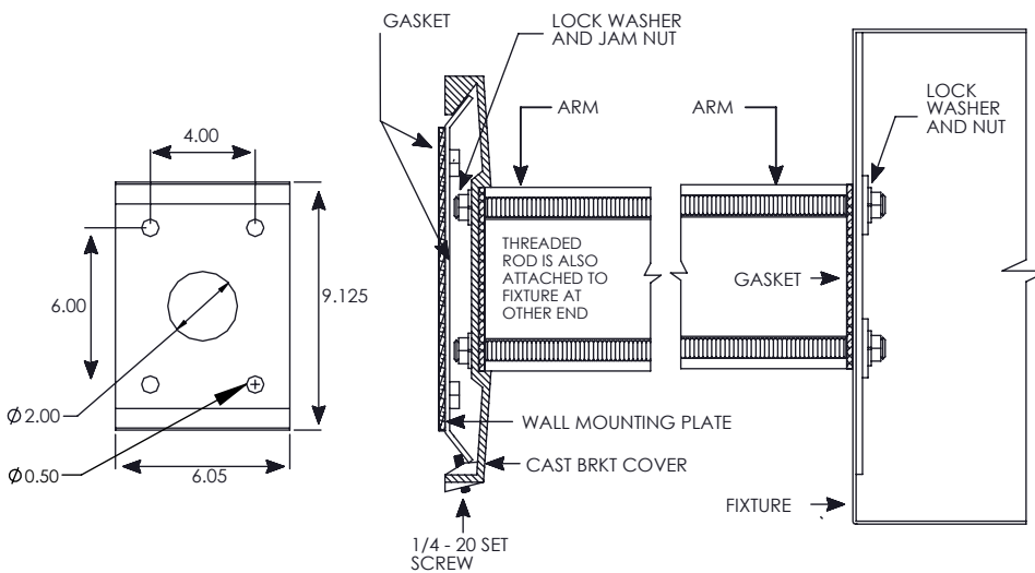
CAST WALL BRACKET
